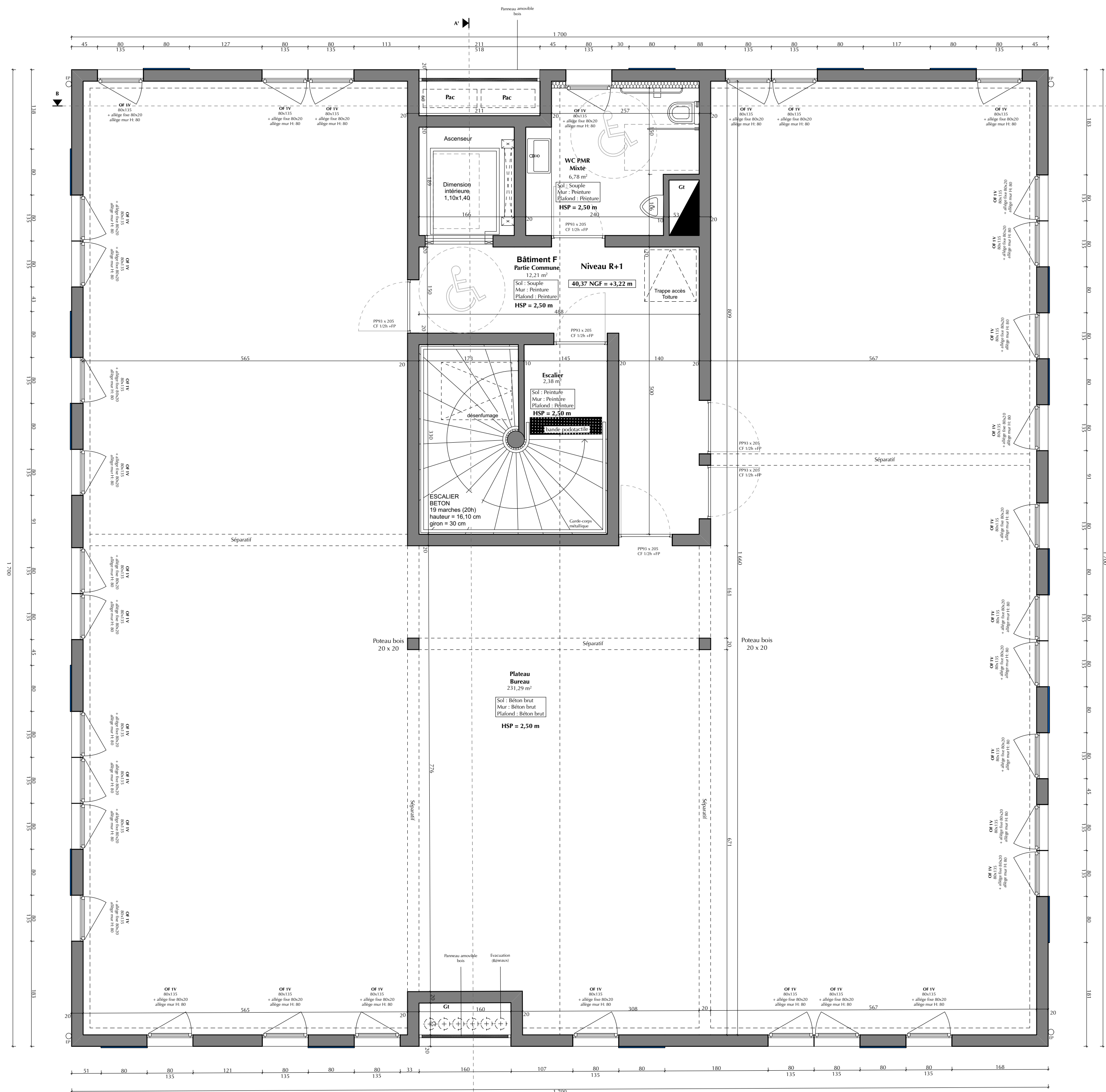
Plan R+1- Ech: 1/50
